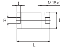
Model OMG-20.../OMG-25...
