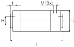
Model OMG-40.../OMG-50.../OMG-100...
