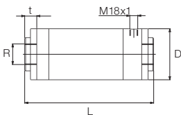
Model OMK-40.../OMK-50...
