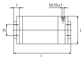
Model OMH-100...
