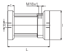
Model OMH-13.../OMH-20.../OMH-25...
