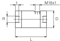
Model OMK-15.../OMK-20.../OMK-25...
