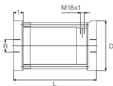
Model OMH-40.../OMH-50...
